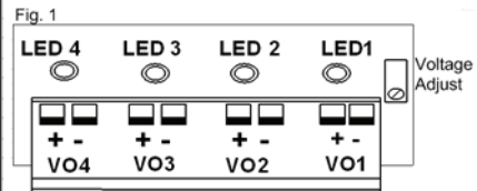
Power Module 1: Output Terminal Block for circuits 1-4 and Voltage
